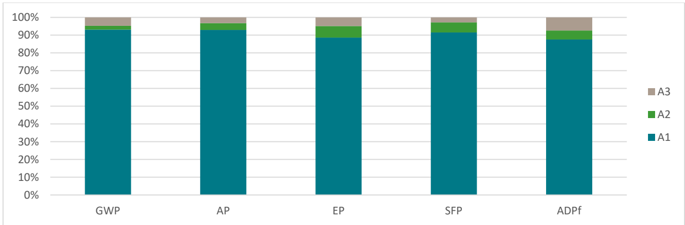
Figure 1: Relative contribution by life cycle stage for 1 metric ton of fabricated HSS
