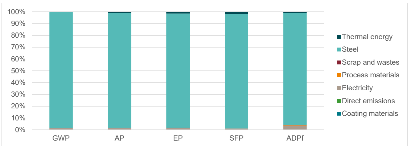
Figure 2: Relative contribution by manufacturing component for 1 metric ton of un-fabricated HSS
